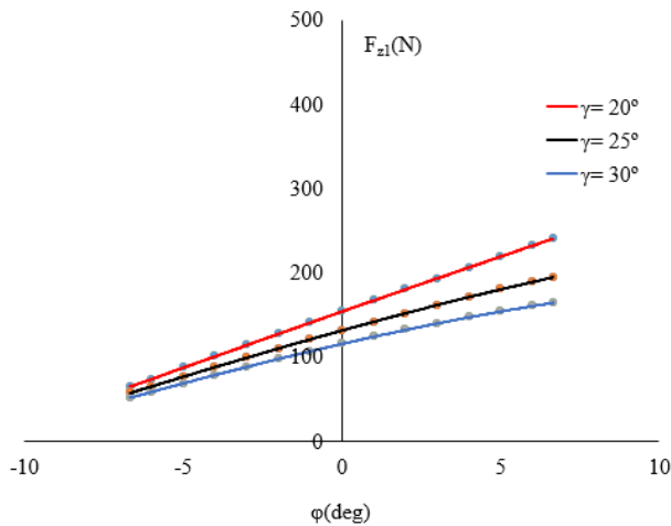
Fig. 6. The contact force on the first link for three values of the profile angle \gamma ( 20^\circ , 25^\circ , 30^\circ ).
