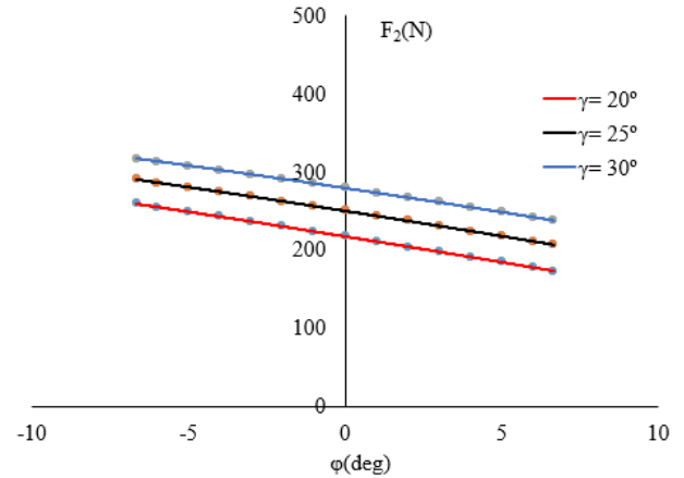
Fig. 4. Tensioning force distribution on the second link for three values of the profile angle \gamma ( 20^\circ , 25^\circ , 30^\circ ).
