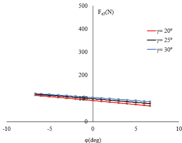
Fig. 8. The contact force distribution on the third link for three values of the profile angle \gamma ( 20^\circ , 25^\circ , 30^\circ ).
