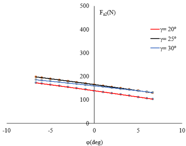
Fig. 7. The contact force distribution on the second link for three values of the profile angle \gamma ( 20^\circ , 25^\circ , 30^\circ ).
