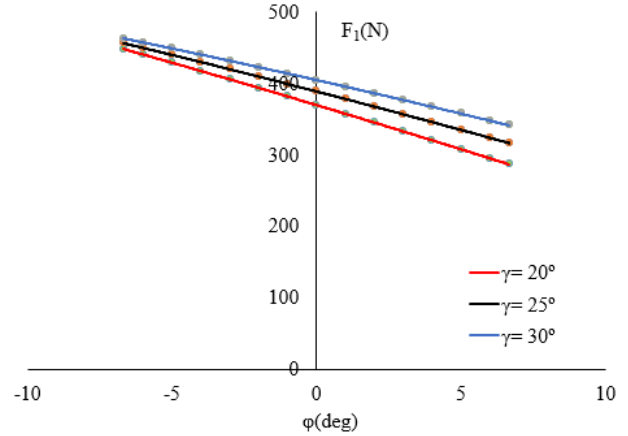
Fig. 3. Tensioning force distribution on the first link for three values of the profile angle \gamma ( 20^\circ , 25^\circ , 30^\circ ).
