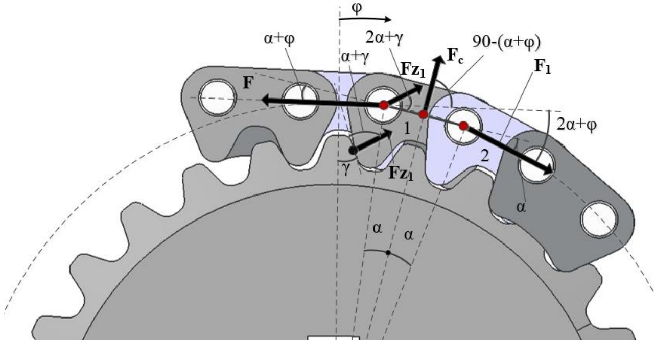
Fig. 2. Force distribution on silent chain transmission.
