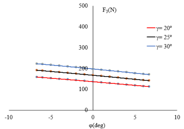
Fig. 5. Tensioning force distribution on the third link for three values of the profile angle \gamma ( 20^\circ , 25^\circ , 30^\circ ).
